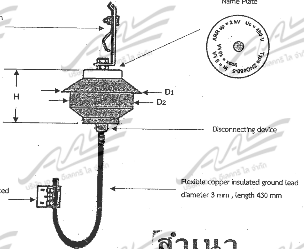
Name Plate
