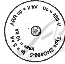
Name Plate
